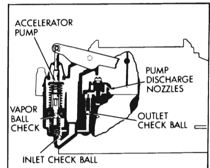
Figure 3-47—Accelerating System
