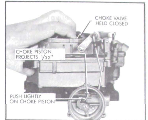
Figure 3-68—Checking Choke Piston Adjustment
