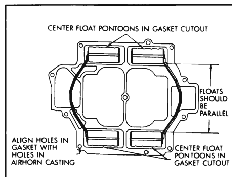
Figure 3-56—Float Alignment
