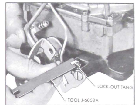
Figure 3-64—Adjusting Secondary Lock-Out
