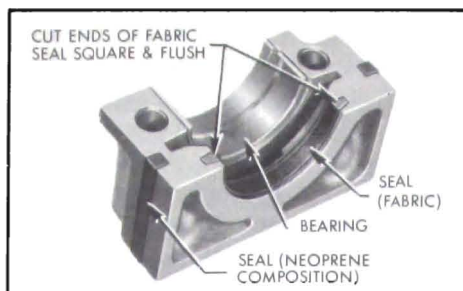
Figure 2-40—Rear Bearing Oil Seals
