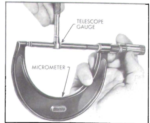
Figure 2-44—Measuring Telescope Gauge
