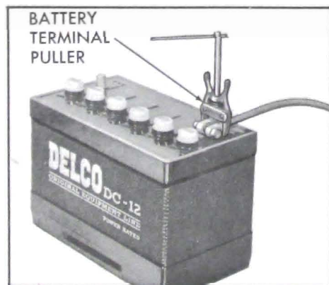
Figure 10-6—Using a Battery Terminal Puller
