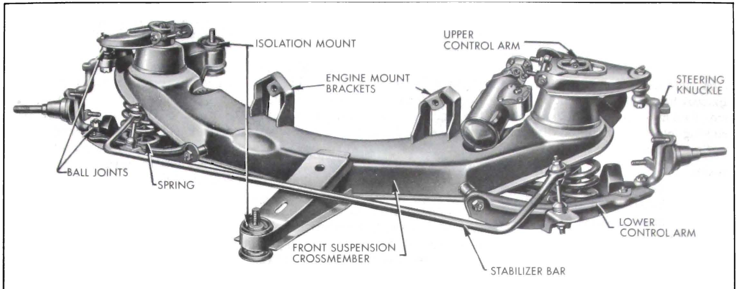
Figure 7-1—Front Suspension
