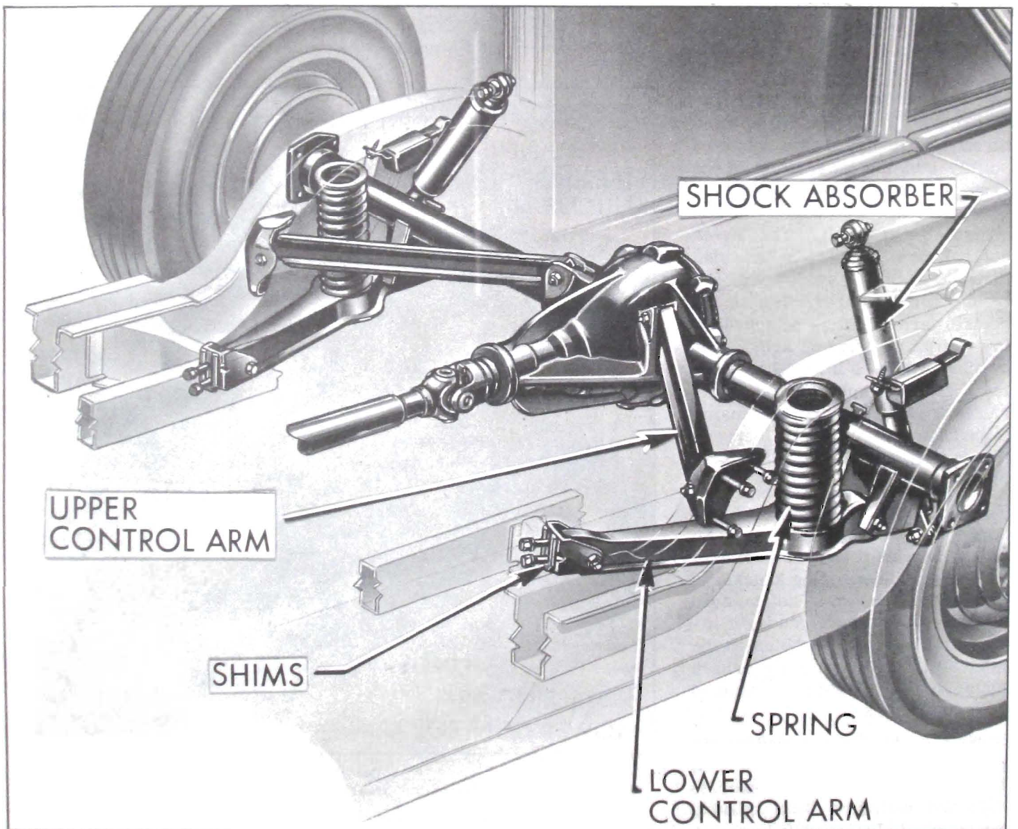
Figure 7-3—Rear Suspension
