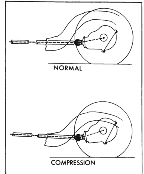
Figure 7-4—Rear Axle Tilting Action
