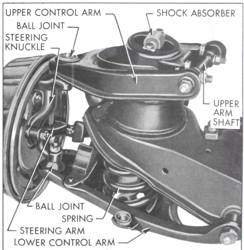
Figure 7-2—Right Steering Knuckle and Ball Joints
