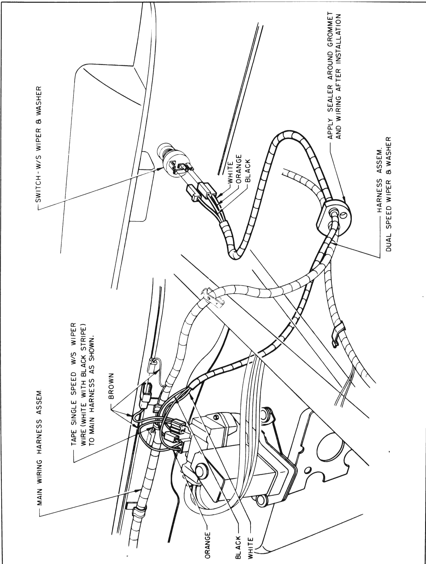
Figure 10-119—Dual Speed Wiper and Washer Wiring
