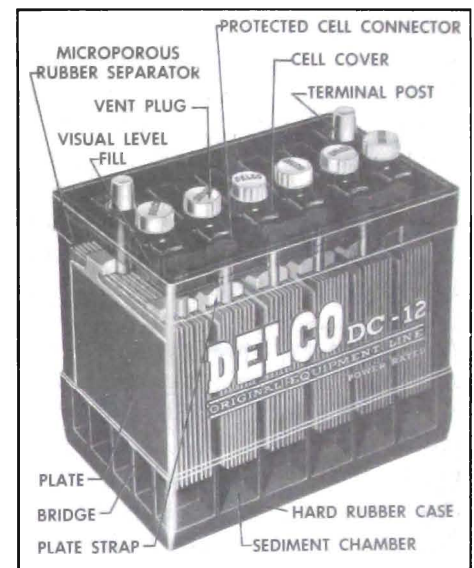
Figure 10-1—Battery
