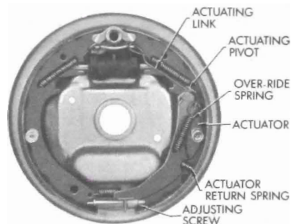
Figure 9-1—Right Rear Wheel Brake Assembly
