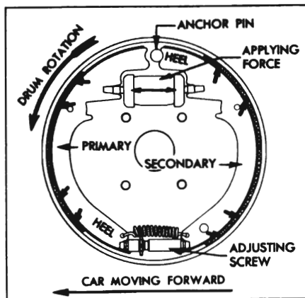
Figure 9-2—Brake Shoe Action
