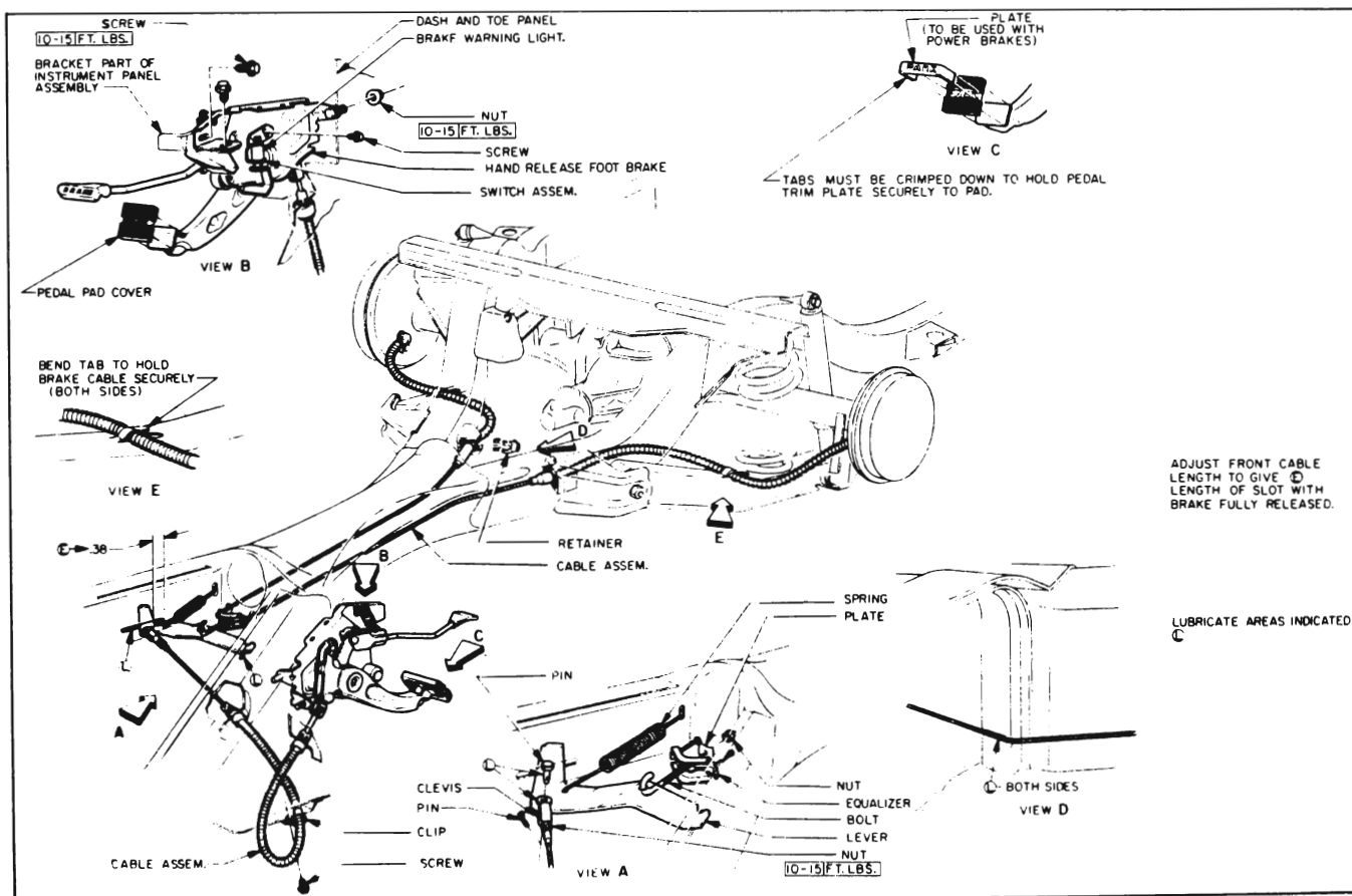
Figure 9-3—Parking Brake Mechanism
