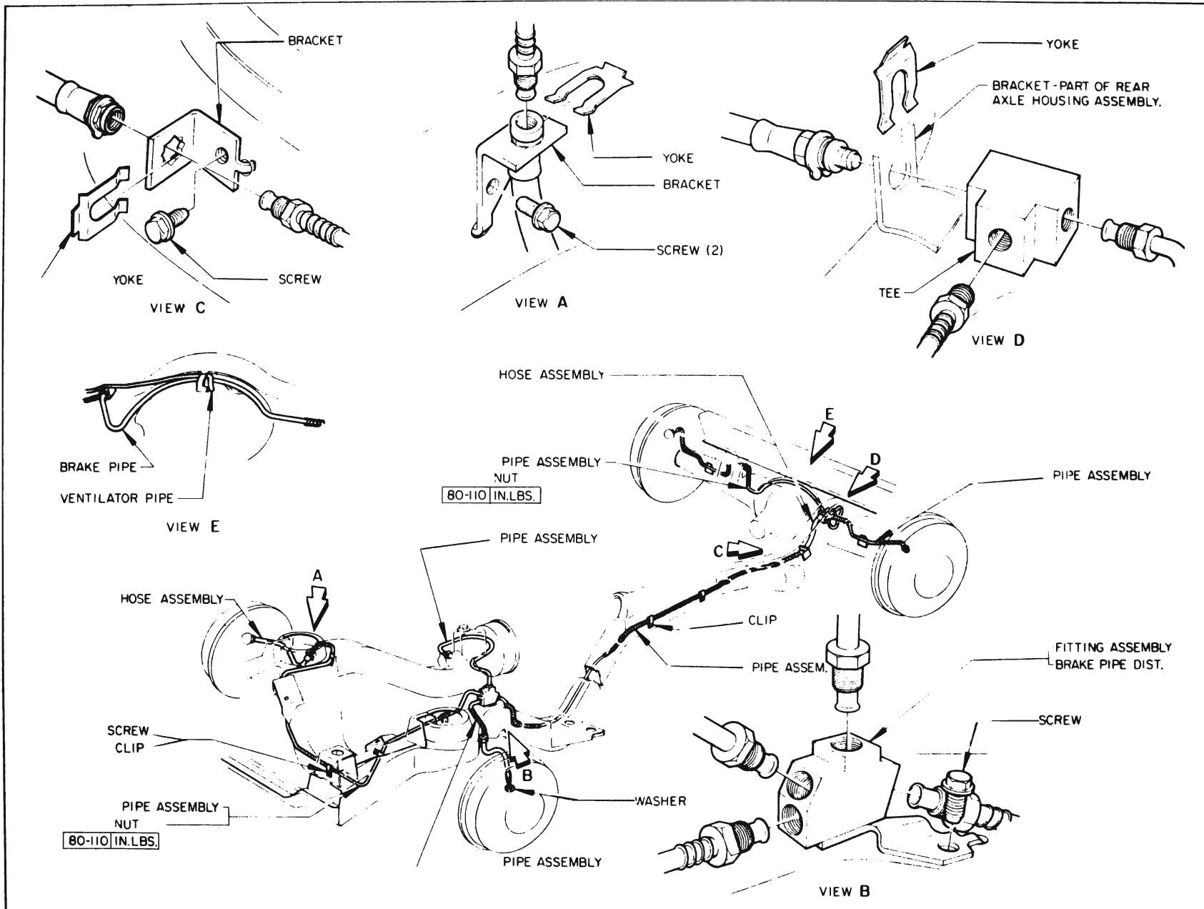
Figure 9-6—Service Brake Control System 4700 Series
