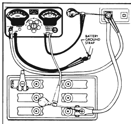
Figure 10-5—Battery Cable Test Connections
