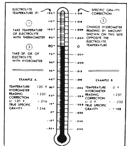
Figure 10-4—Specific Gravity Temperature Correction Scale
