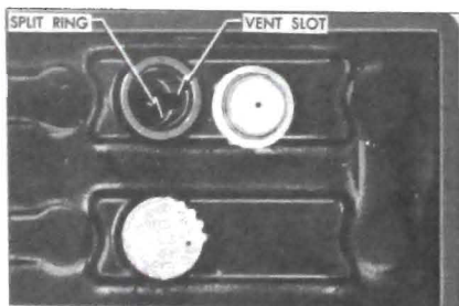
Figure 10-2—Battery Filler Well
