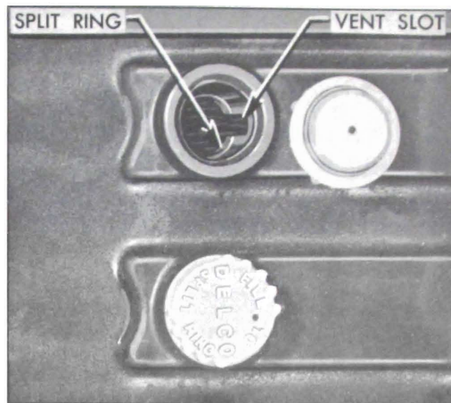
Figure 10-2—Battery Filler Well
