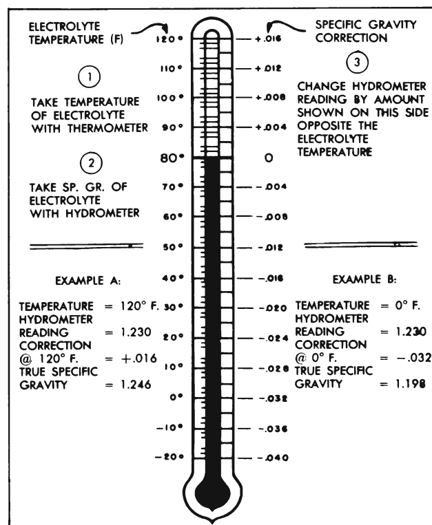
Figure 10-4—Specific Gravity Temperature Correction Scale
