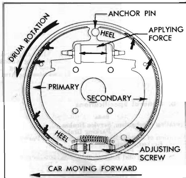
Figure 9-2—Brake Shoe Action
