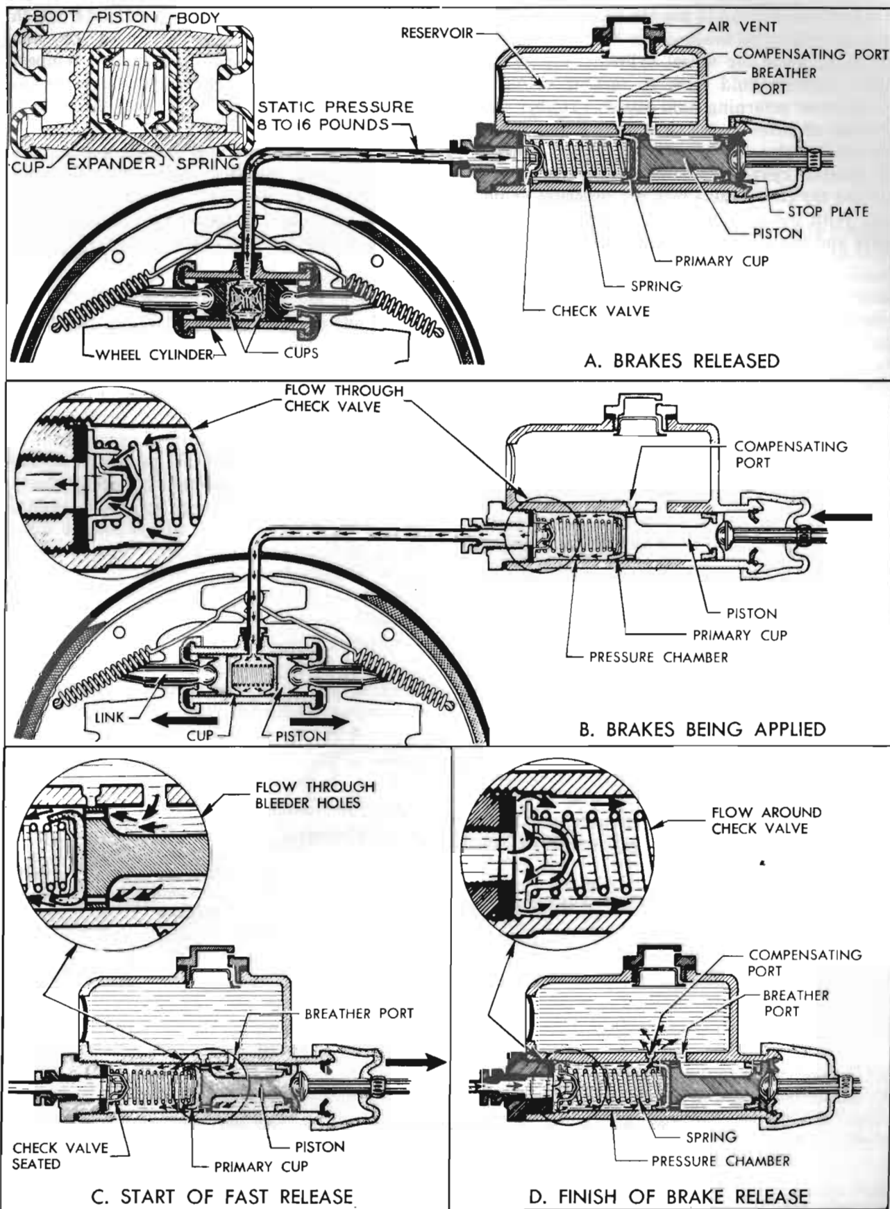
Figure 9-5—Hydraulic Components
