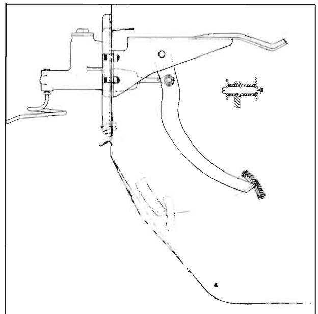
Figure 9-4—Mounting of Brake Master Cylinder and Pedal
