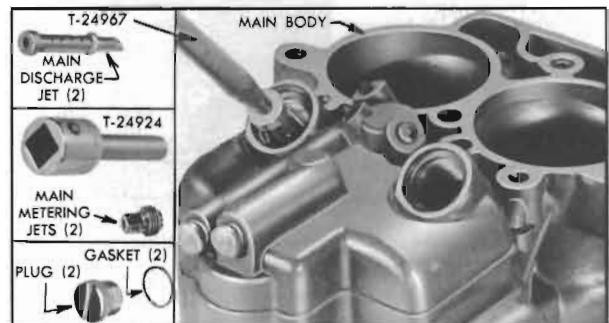
Figure 3-71—Removing Main Metering Well Parts
