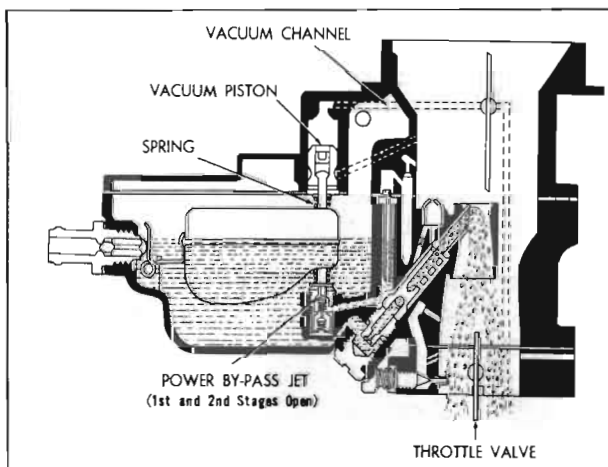
Figure 3-63—Power System
