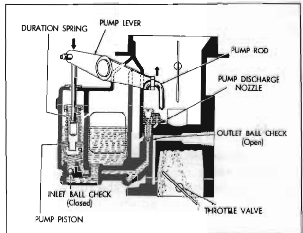
Figure 3-64—Accelerating System
