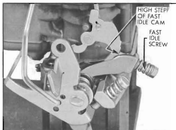
Figure 3-74—Fast Idle Speed Adjustment
