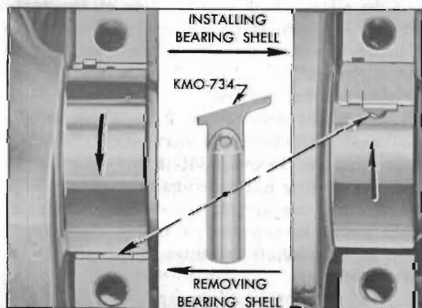
Figure 2-31—Removing and Installing Crankshaft Bearing Upper Shell
