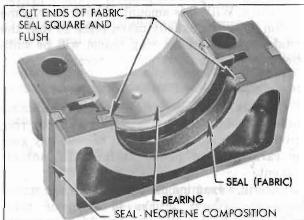
Figure 2-32—Rear Bearing Oil Seals (364 Rear Bearing Cap Shown)
