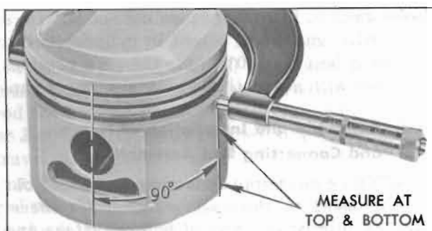
Figure 2-35—Measuring Piston with Micrometer
