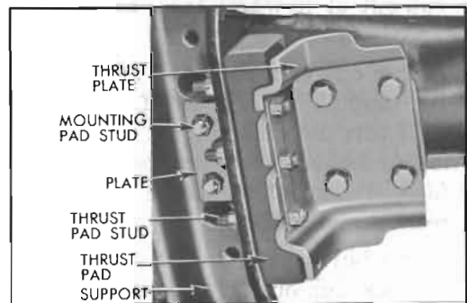
Figure 2-41—Transmission Mounting—Bottom View
