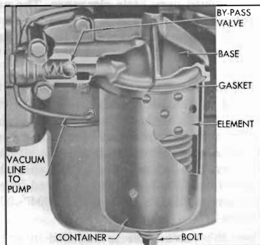
Figure 2-9—Oil Filter Installation
