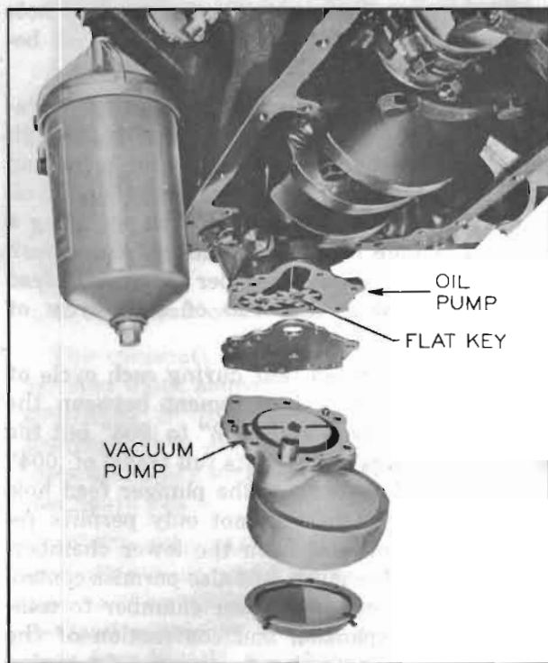
Figure 2-8—Oil and Vacuum Pump and Screen
