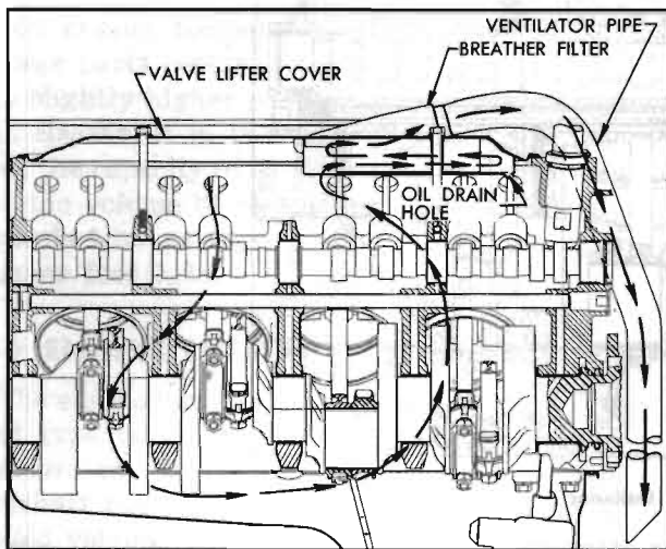
Figure 2-12—Crankcase Ventilation
