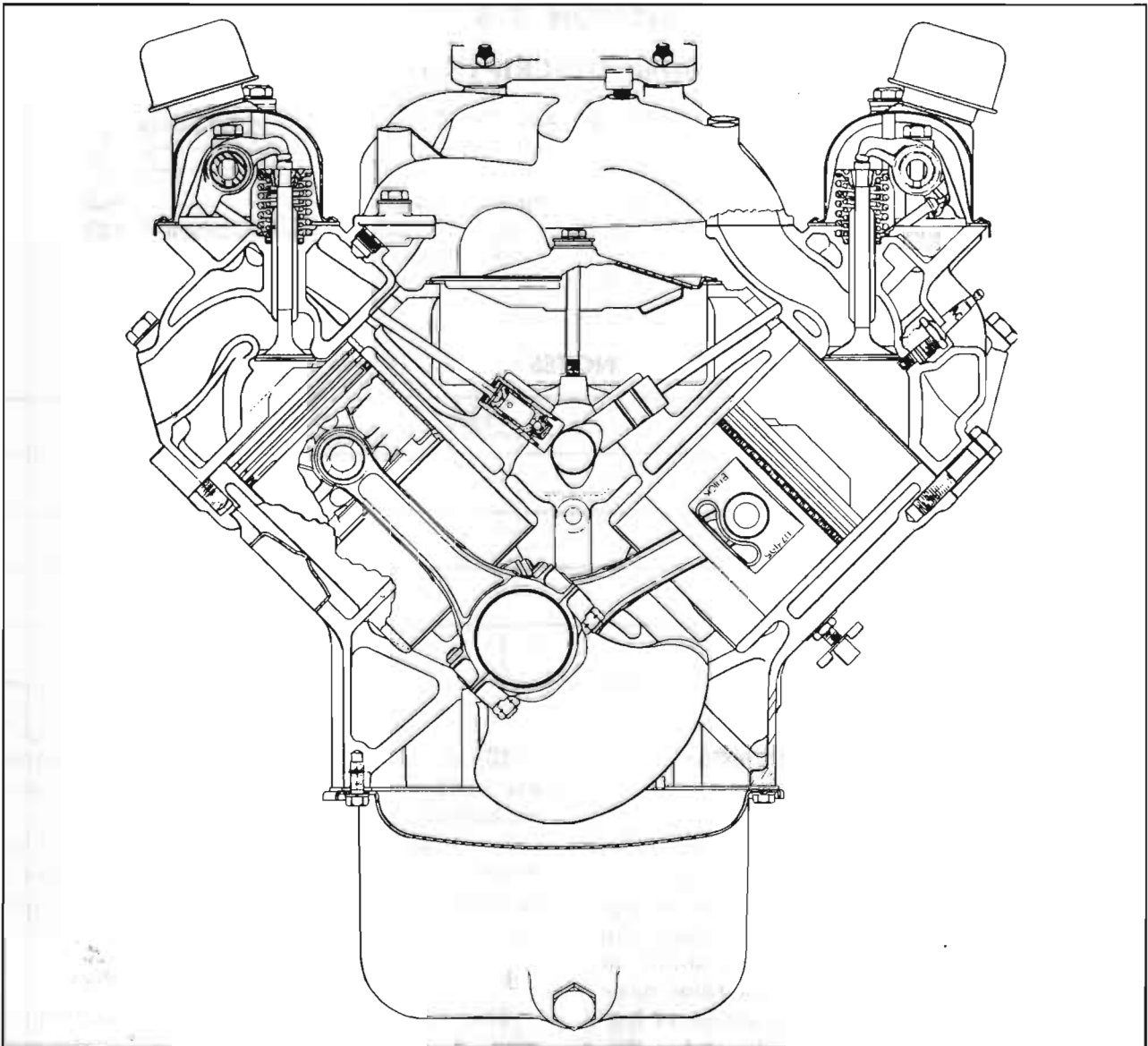
Figure 2-2—Engine, End Sectional View—All Series
