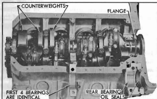
Figure 2-4—Crankshaft and Bearings
