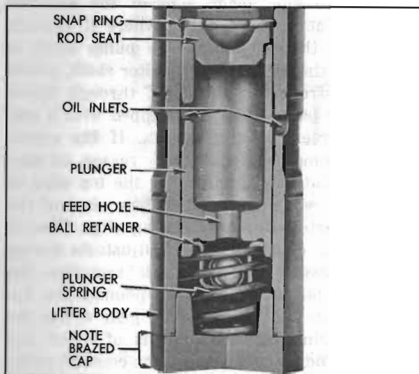
Figure 2-7—Hydraulic Valve Lifter, with Quarter Sections Cut Out
