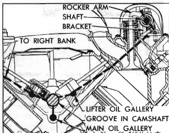
Figure 2-11—Oil Supply to Lifters, Rocker Arms and Valves
