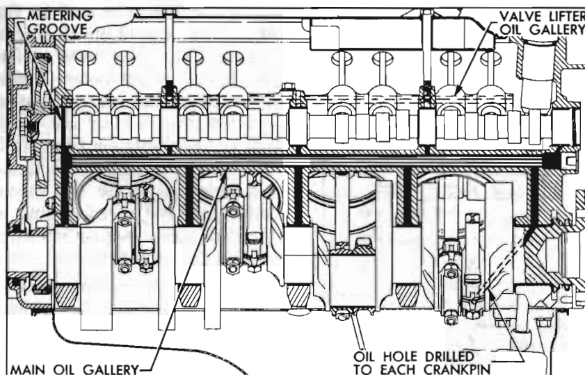
Figure 2-10—Oil Galleries
