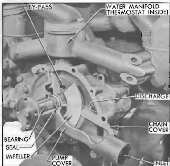
Figure 2-14—Water Pump Installation
