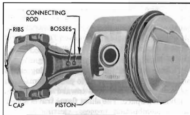
Figure 2-5—Connecting Rod and Piston Assembly
