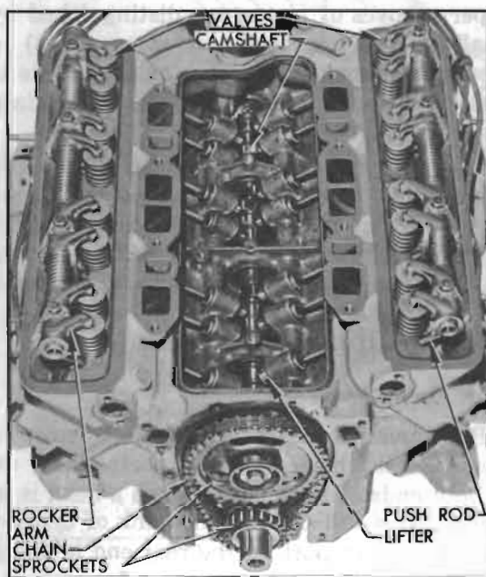
Figure 2-6—Valve Mechanism
