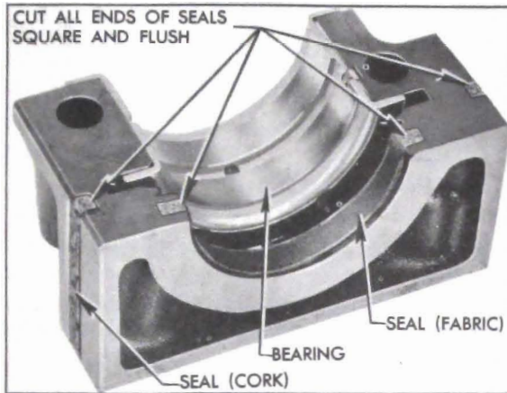
Figure 2-29—Rear Bearing Oil Seals
