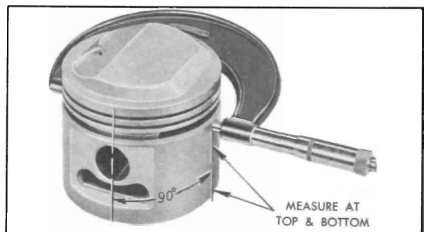
Figure 2-32—Measuring Piston with Micrometer
