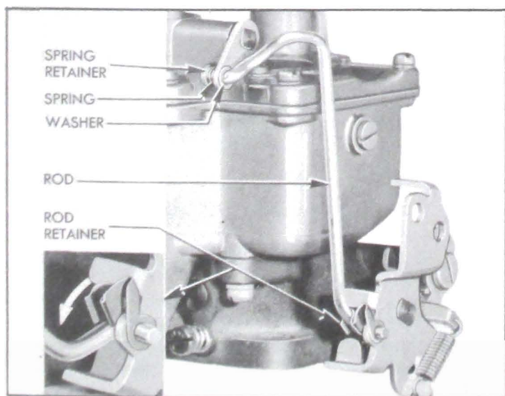
Figure 3-37—Installation of Throttle Connector Rod
