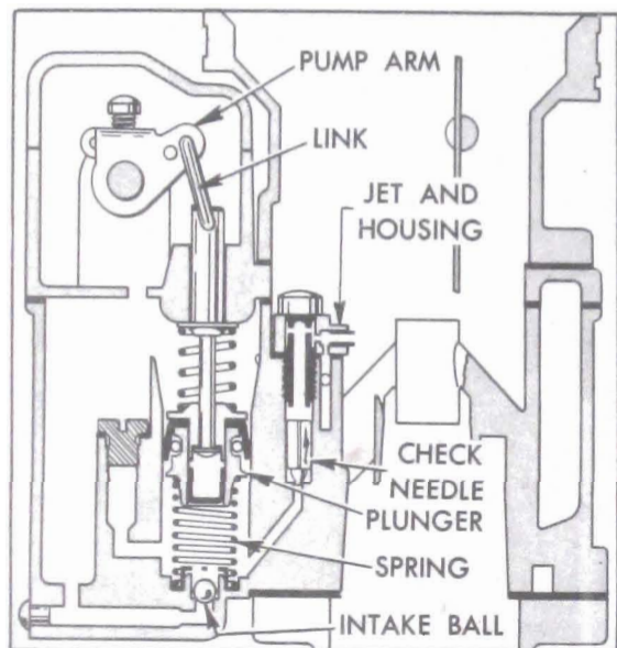
Figure 3-22—Accelerating System—Carter WCD Carburetor
