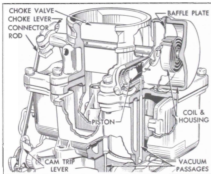
Figure 3-23—Carter Climatic Control
