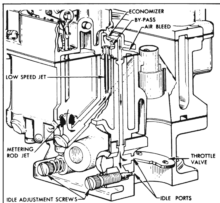
Figure 3-20—Low Speed System—Carter WCD Carburetor
