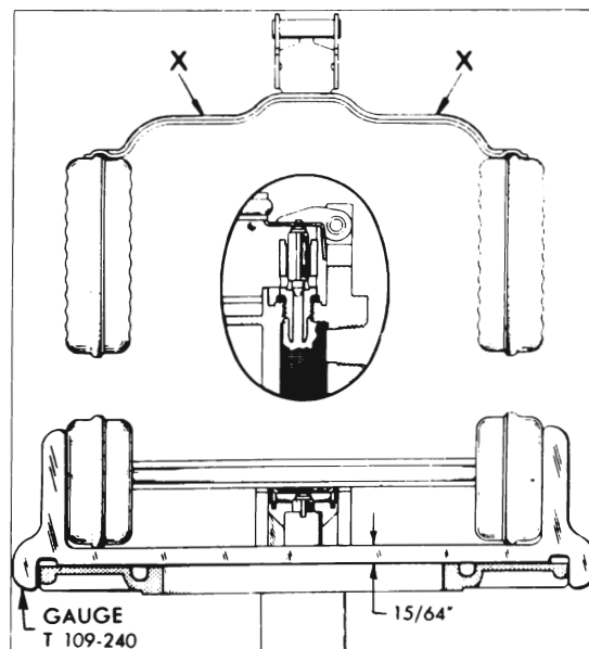
Figure 3-36—Checking Float with Gauge
