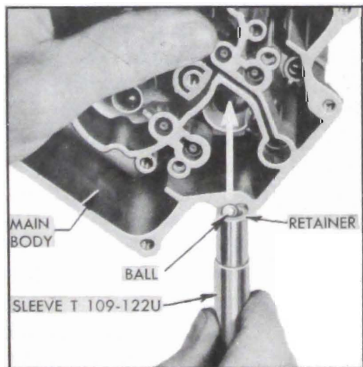
Figure 3-35—Installation of Intake Check Ball and Retainer
