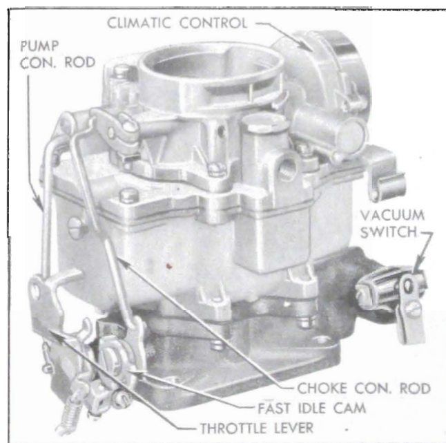
Figure 3-18—Carter WCD Carburetor Assembly
