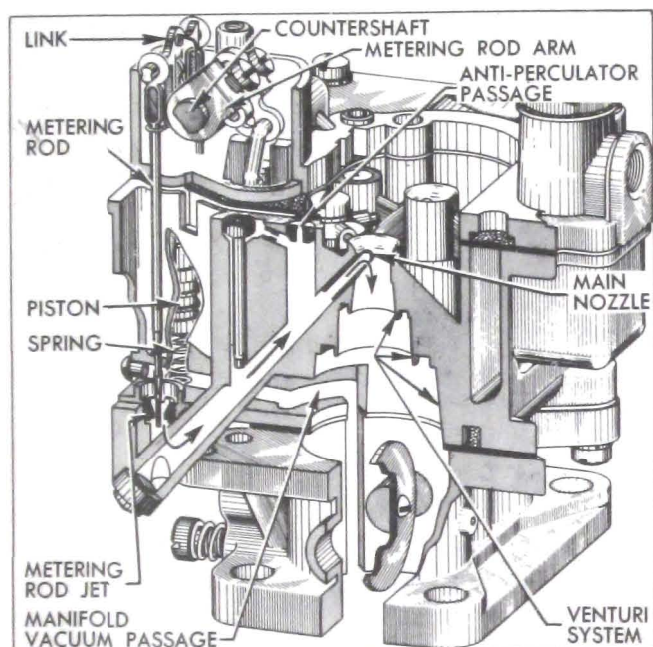
Figure 3-21—High Speed and Power Systems—Carter WCD Carburetor
