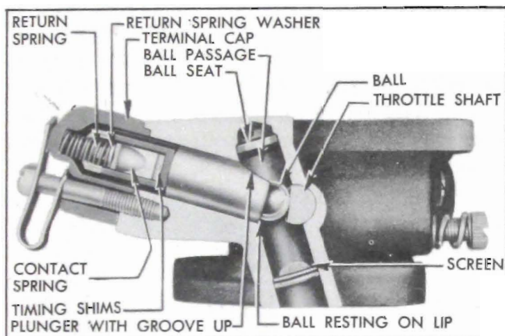
Figure 3-34—Correct Installation of Switch Parts
