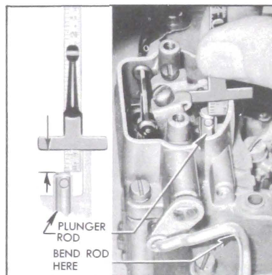
Figure 3-38—Checking Pump Plunger Adjustment with Scale
