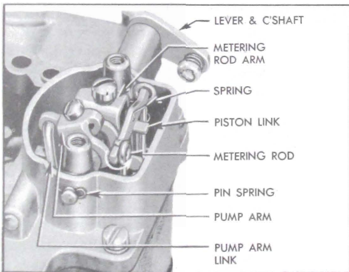
Figure 3-28—Removal of Metering Rods and Operating Parts
