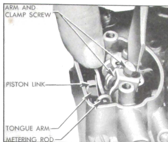
Figure 3-39—Adjusting Metering Rods
