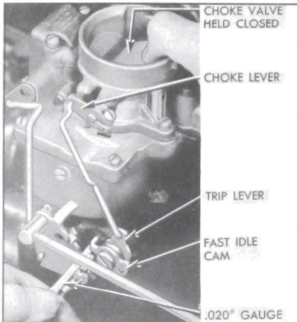
Figure 3-24—Checking Carter Fast Idle Cam Clearance
