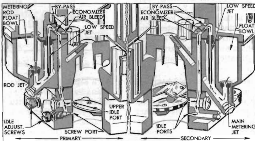
Figure 3-44—Primary and Secondary Low Speed Systems—WCFB Carter
