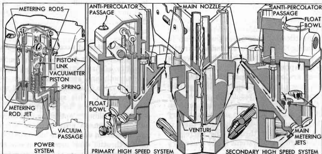
Figure 3-45—High Speed and Power Systems—WCFB Carter
