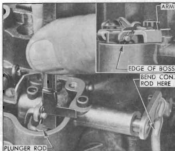
Figure 3-55—Checking Pump Plunger Adjustment
