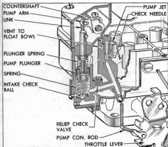
Figure 3-46—Accelerating System—WCFB Carter
