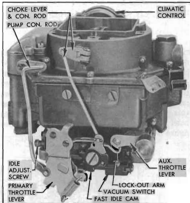
Figure 3-42—Carter WCFB Carburetor Assembly
