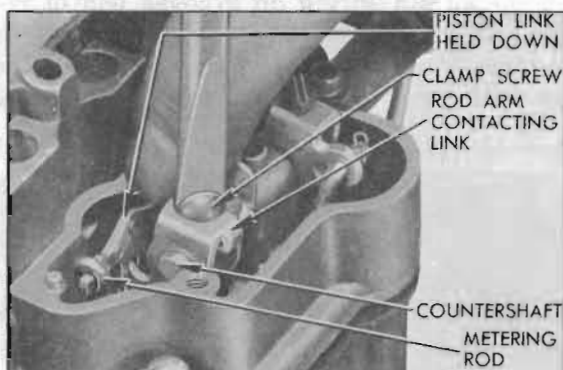
Figure 3-56—Metering Rod Adjustment
