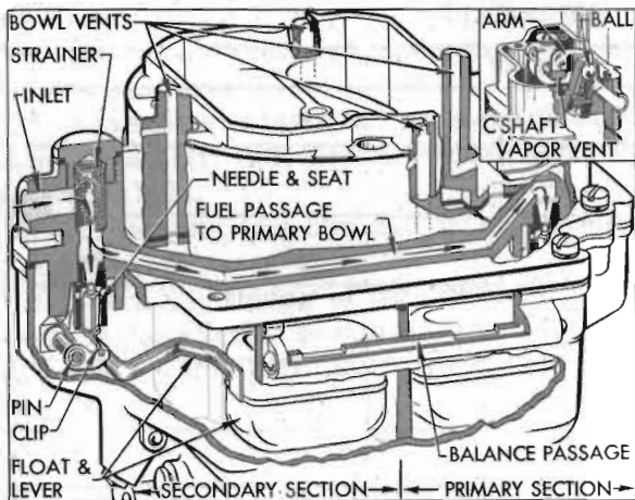
Figure 3-43—Primary and Secondary Float Systems—WCFB Carter
