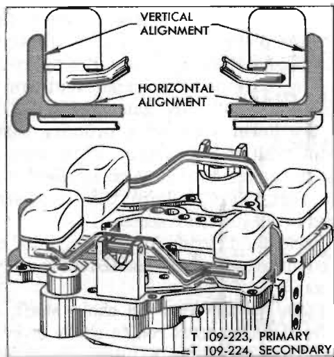
Figure 3-54—Checking Float Adjustment With Gauge
