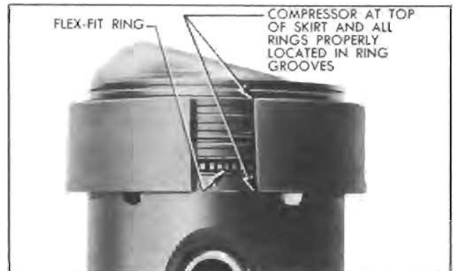
Figure 2-33—Rings Held in Place by Compressor
