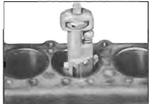
Figure 2-26—Removing Ridge from Cylinder Bore
