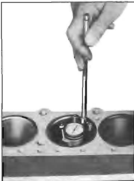
Figure 2-28—Checking Cylinder Bore with Gauge
