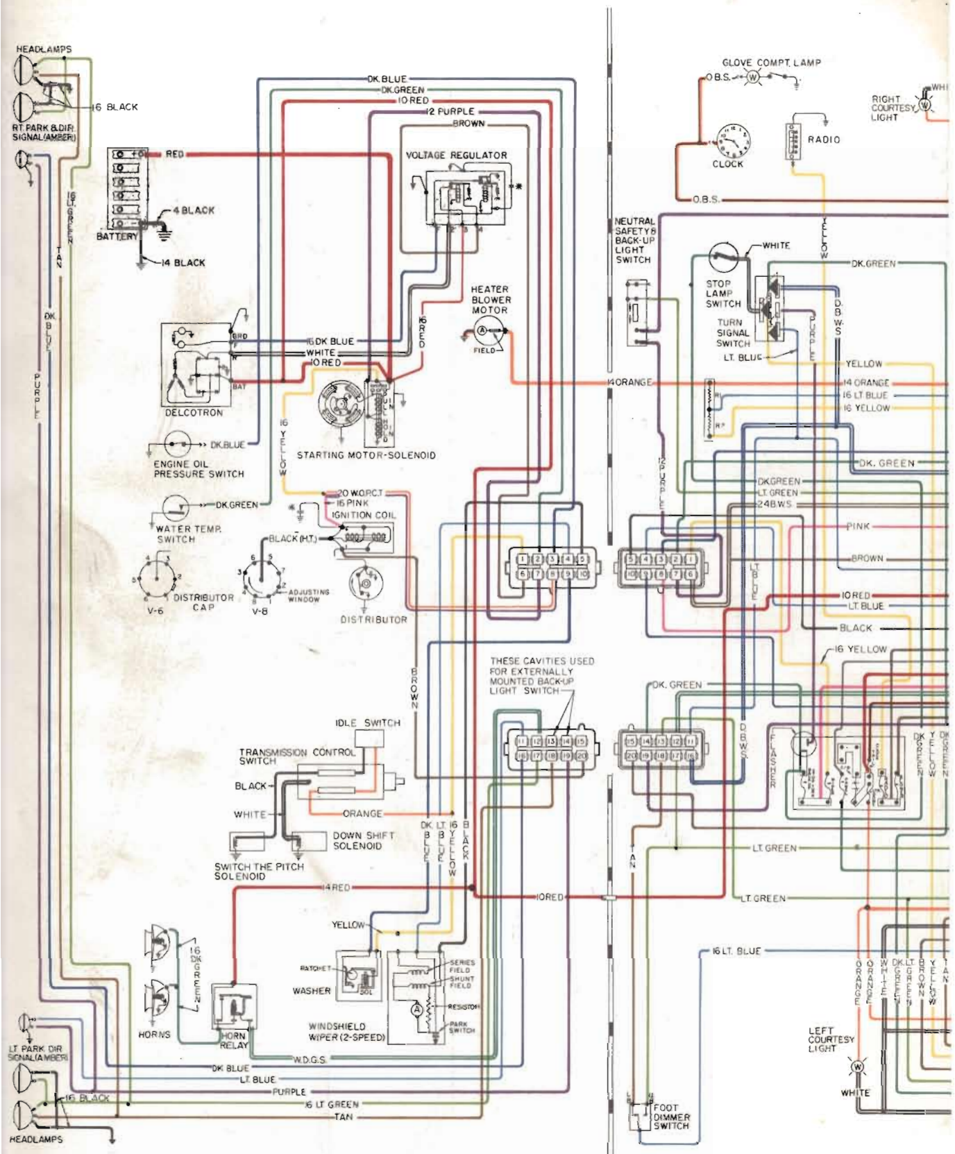
Figure 120-154—Special Wiring Circuit Diagram
