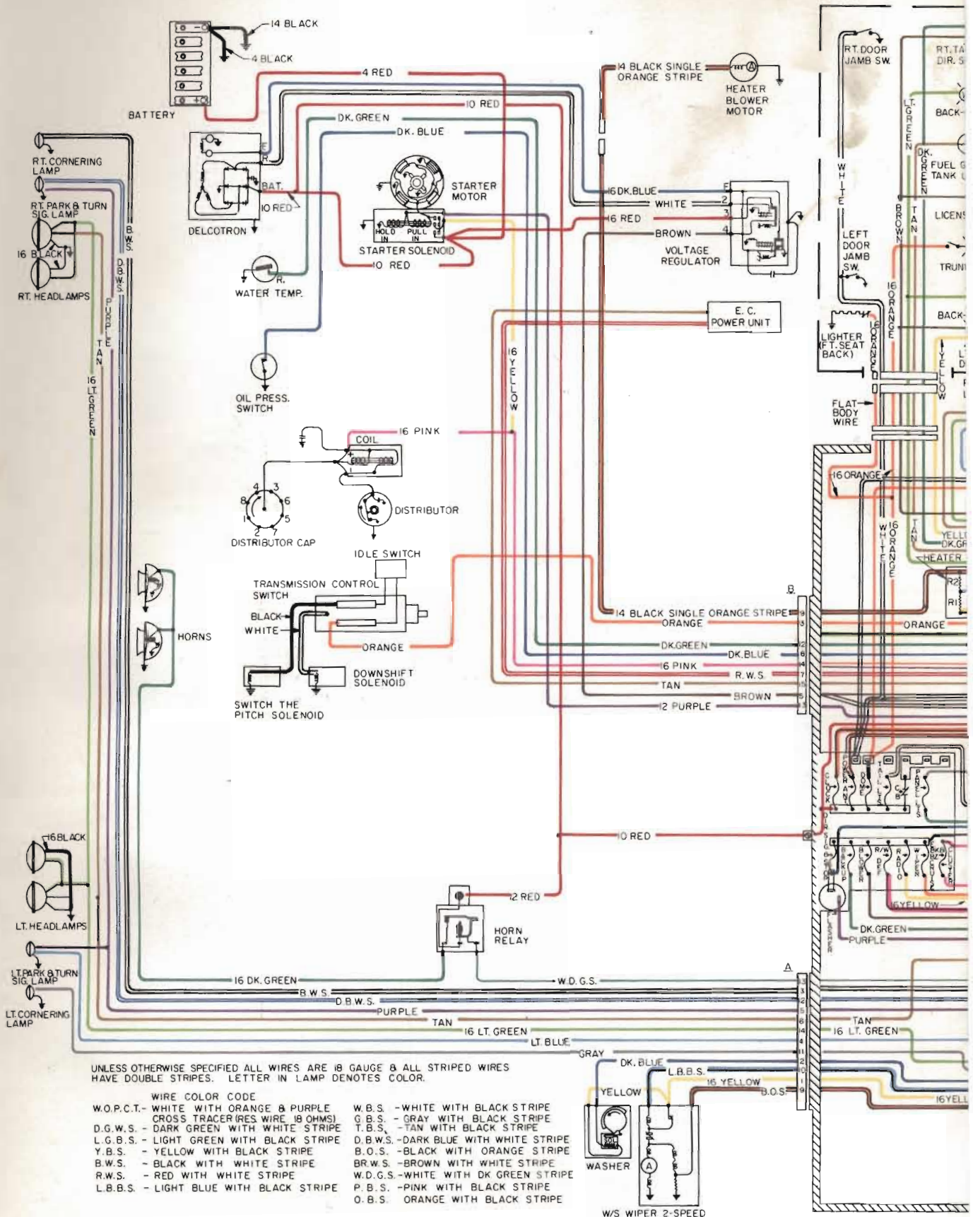
Figure 120-156—LeSabre Wiring Circuit Diagram
