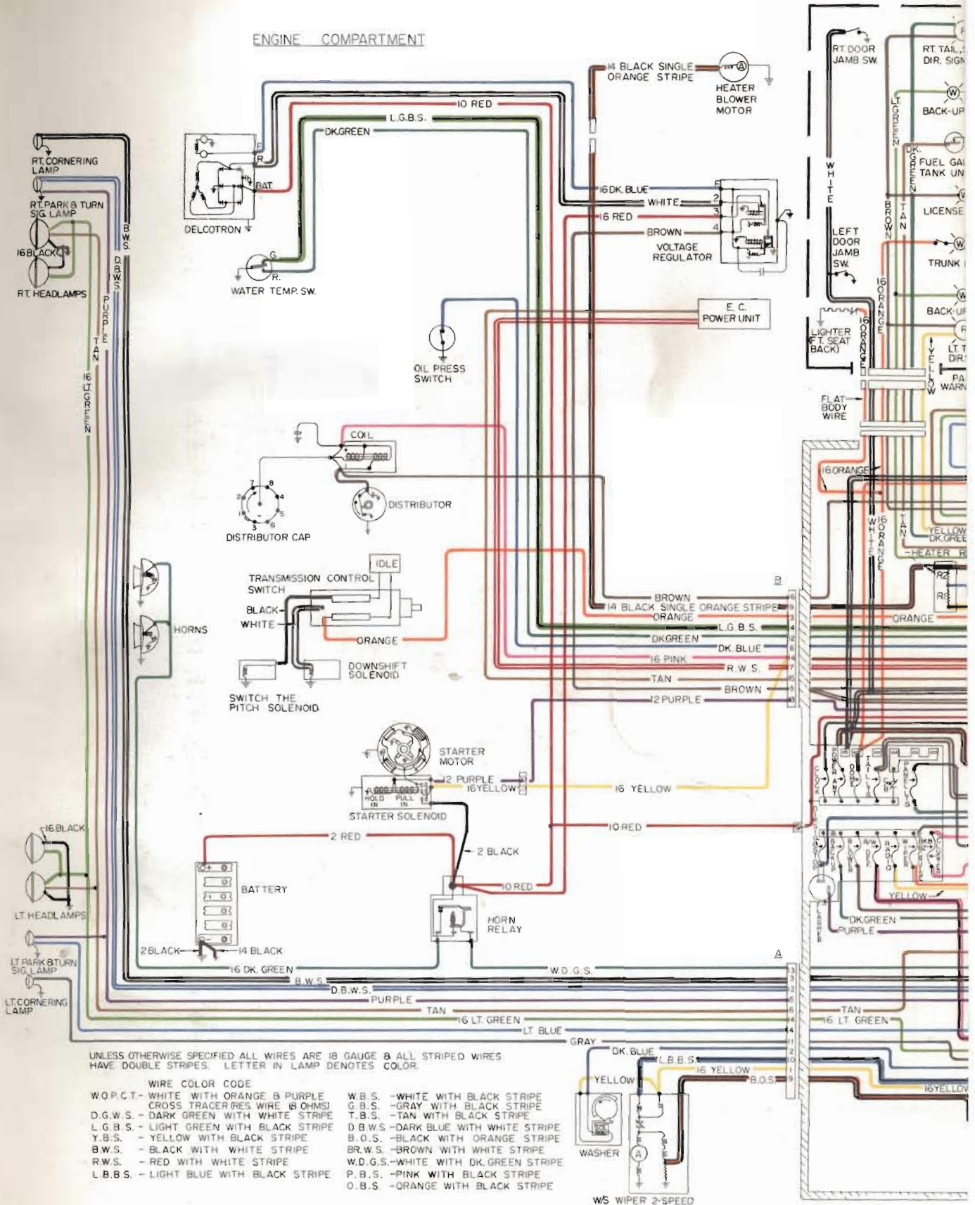
Figure 120-157—Wildcat & Electra Wiring Circuit Diagram
