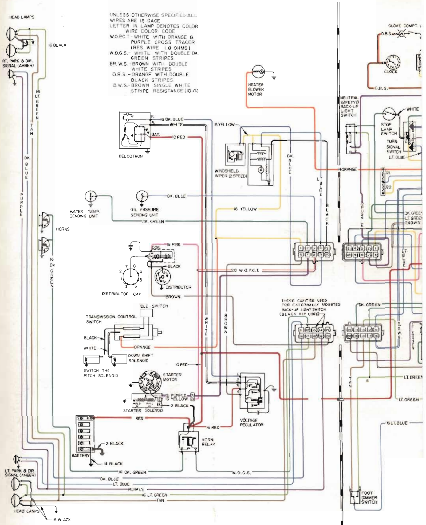
Figure 120-155—Skylark Gran Sport Wiring Circuit Diagram
